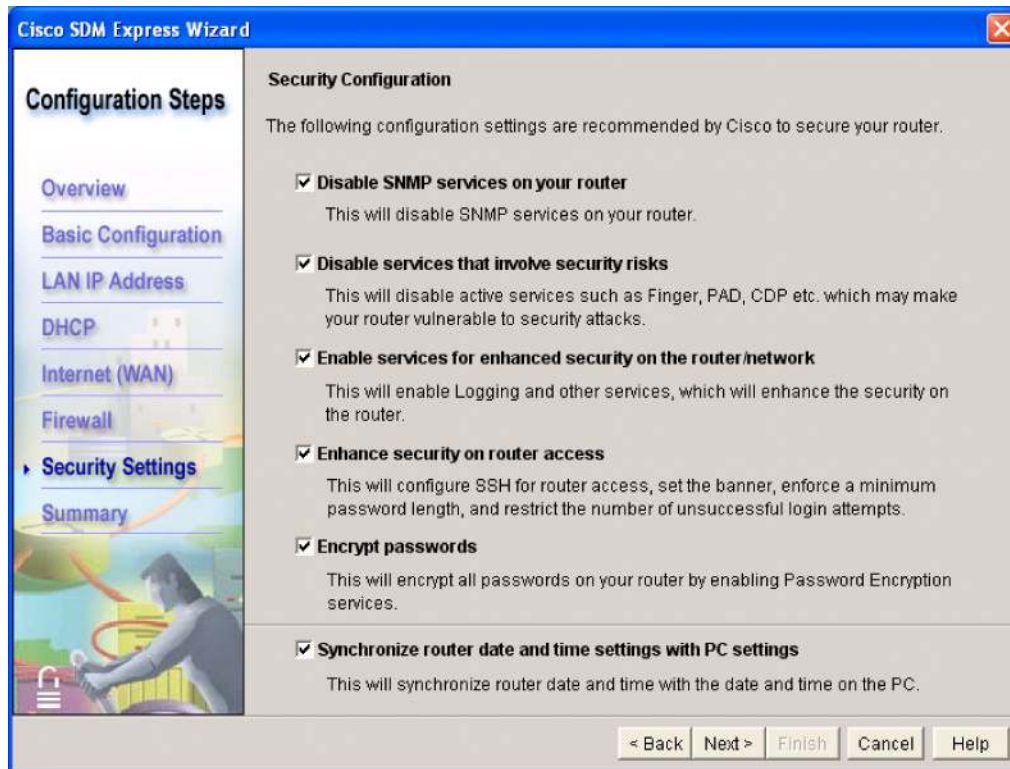
Figure 3. Cisco SDM
